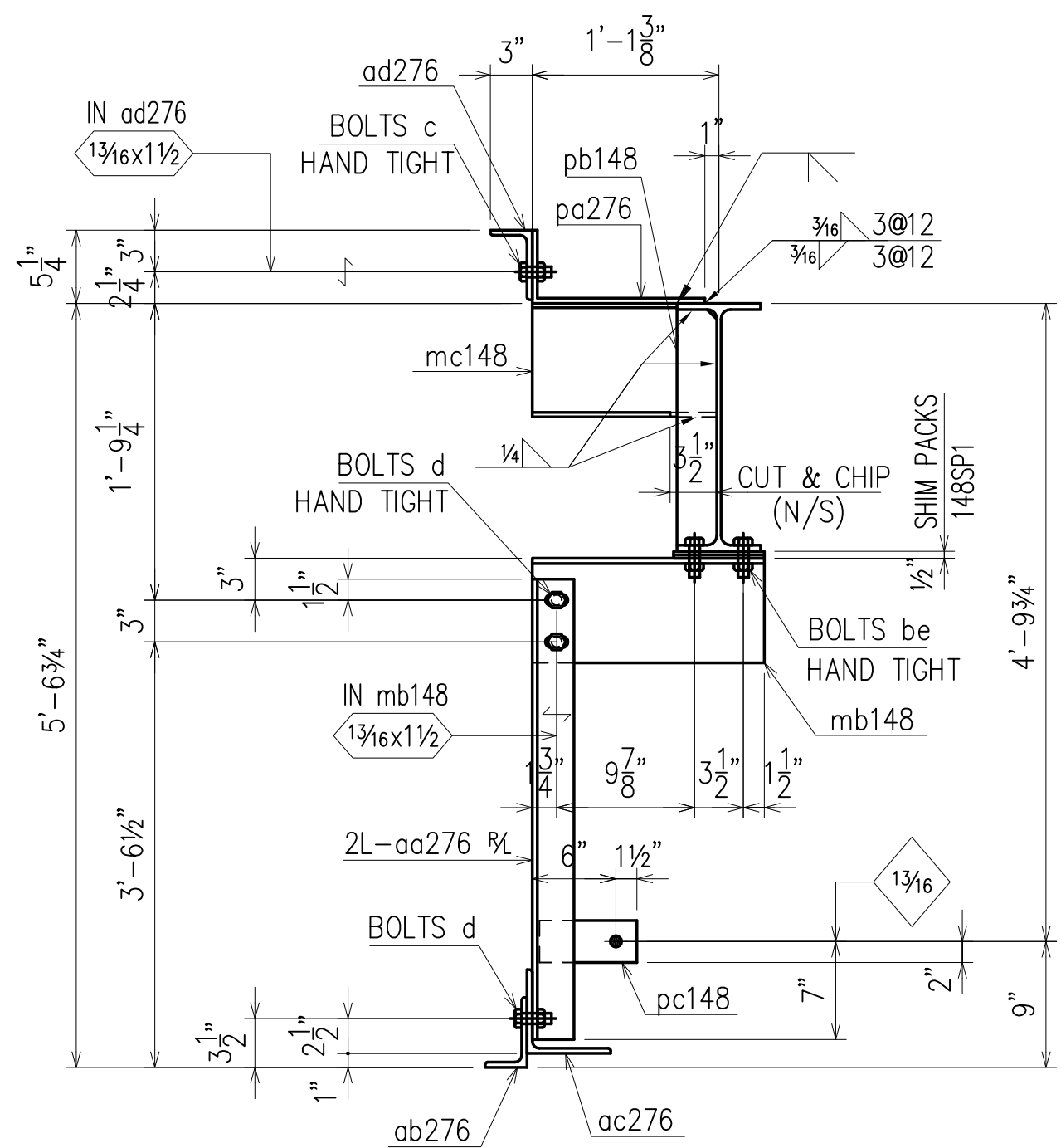
SECTION 2
